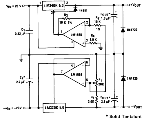
FIGURE 7.18. Variable Tracking Dual Supply \pm 5.0\text{ V} - \pm 18\text{ V}
