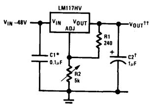
1.2V–45V Adjustable Regulator
