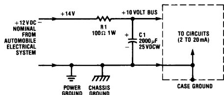
FIGURE 1. Basic Decoupling for Low-Power Application
