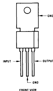
Plastic Package
