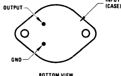
Steel Metal Can Package TO-3 (K)
