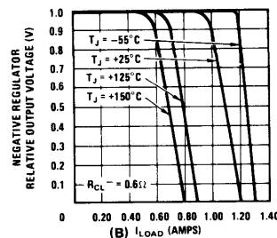
FIGURE 7.24. External Current Limiting Characteristics-Boosted
