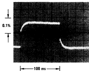
LM137, V_{OUT} = -10V V_{IN} - V_{OUT} = -40V I_L = 0A \rightarrow 0.25A \rightarrow 0A Horizontal sensitivity, 20 ms/div FIGURE 2
