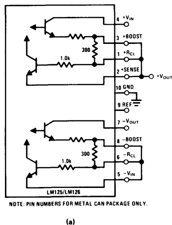
FIGURE 7.19 (a). Basic Dual Regulator.
