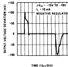
LM126 Line Transient Response
