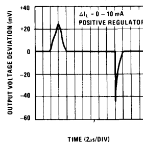
LM126 Load Transient Response
