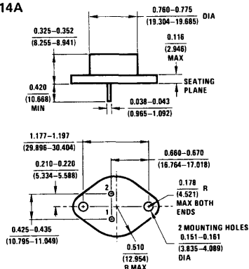
TO-3 STEEL Metal Can NS Package Number K02A
