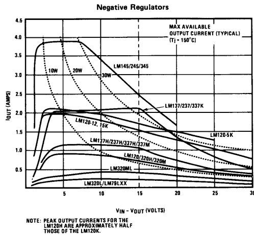
FIGURE 3.2. Max Available Output Current at T_j = 150^\circ\text{C}
