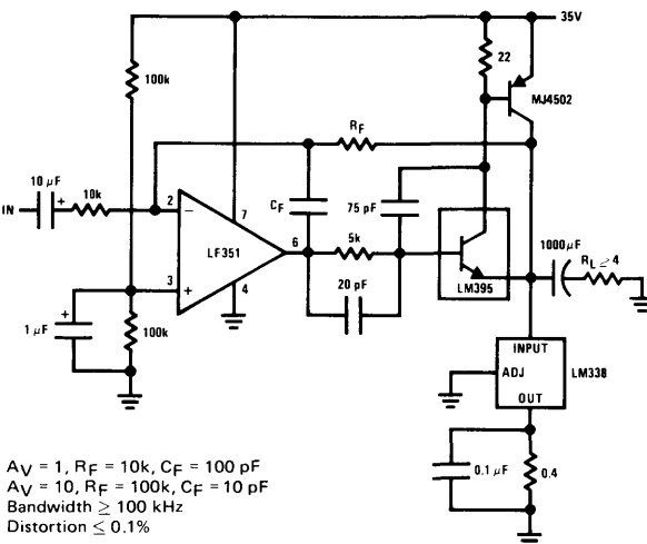
Power Amplifier
