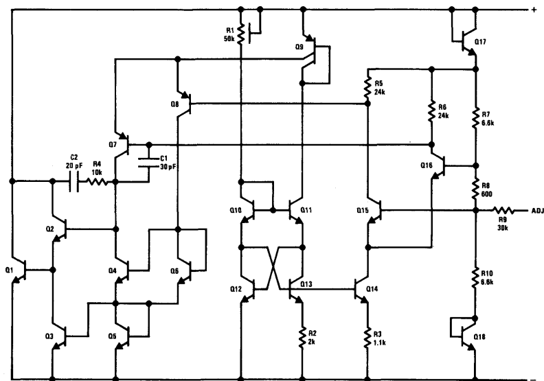
2.5V Reference
