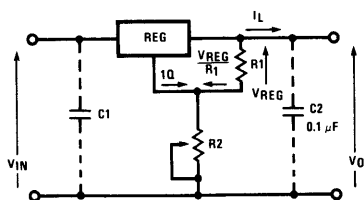
FIGURE 7.5. Adjustable V_{OUT}
