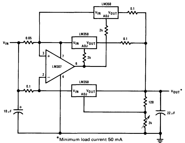
10A Regulator
