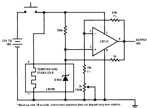
Portable Calibrator*
