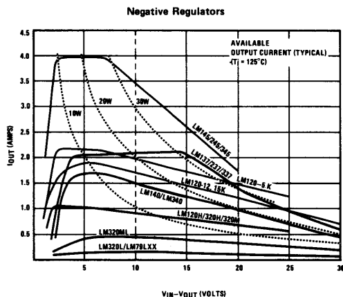
FIGURE 3.1. Max Available Output Current at T_J = 125^\circ\text{C}
