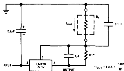
Current Source
