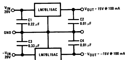
\pm 15\text{V} , 100 mA Dual Power Supply
