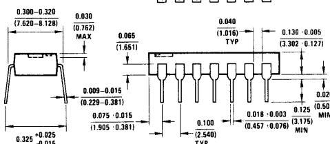
Molded Plastic Dual-in-Line NS Package Number N14A
