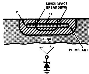
FIGURE A3.3. Zener (avalanche) Reference Employing Ion Implantation to Produce a Subsurface Breakdown
