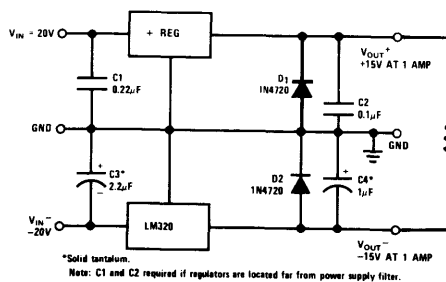
FIGURE 7.15. Dual Power Supply
