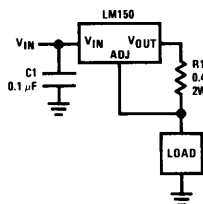
3A Current Regulator
