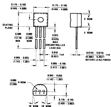
TO-92 Molded Plastic NS Package Number Z03A
