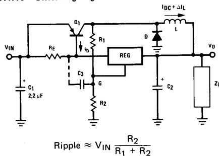
FIGURE 7.13. Switching Regulator
