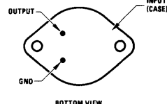
Aluminum Metal Can Package TO-3 (KC)
