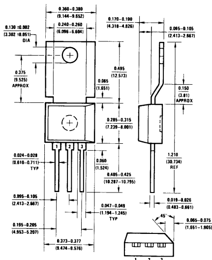
T-202 Molded (T) NS Package Number PO3E
