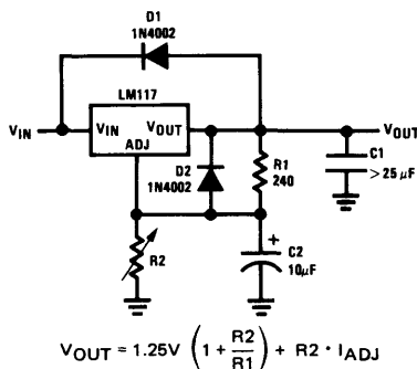
FIGURE 4. Regulator with Protection Diodes Against Capacitor Discharge
