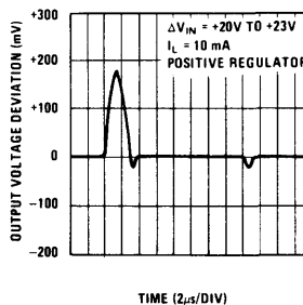
LM126 Line Transient Response
