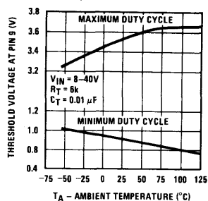
Maximum and Minimum Duty Cycle Threshold Voltage
