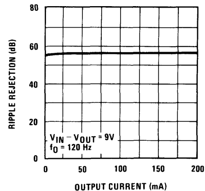
Ripple Rejection
