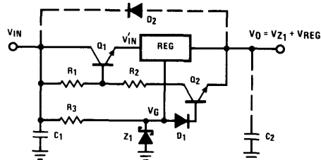
FIGURE 7.10. High-Voltage Regulator
