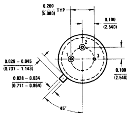
TO-39 Metal Can (H) NS Package Number H03G
