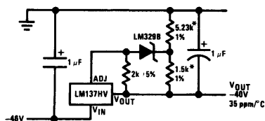
High Stability -40\text{V} Regulator
