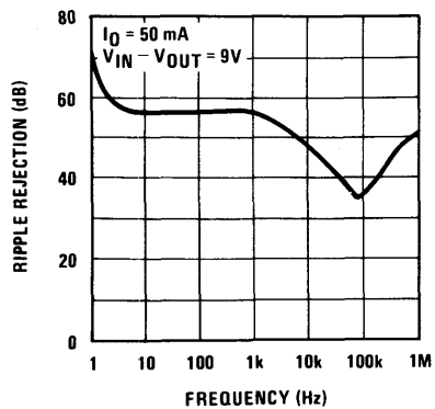
Ripple Rejection
