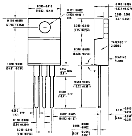
TO-220 Molded (T) NS Package Number T03B
