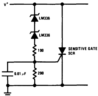
5V Crowbar
