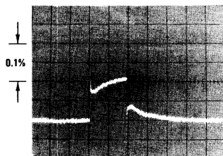
LM137, V_{OUT} = -10V V_{IN} - V_{OUT} = -40V I_L = 0A \rightarrow 0.25A \rightarrow 0A Vertical sensitivity, 5 mV/div FIGURE 1
