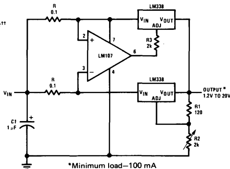
10A Regulator
