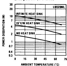
Maximum Average Power Dissipation (TO-202)
