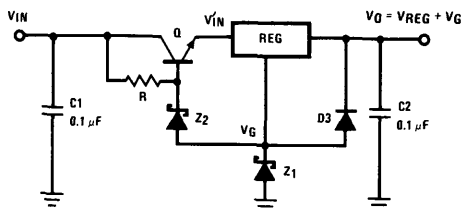
FIGURE 7.9. High-Voltage Regulator
