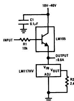
Power Follower
