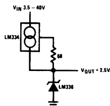
Wide Input Range Reference
