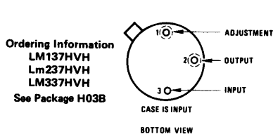
TO-5 Metal Can Package
