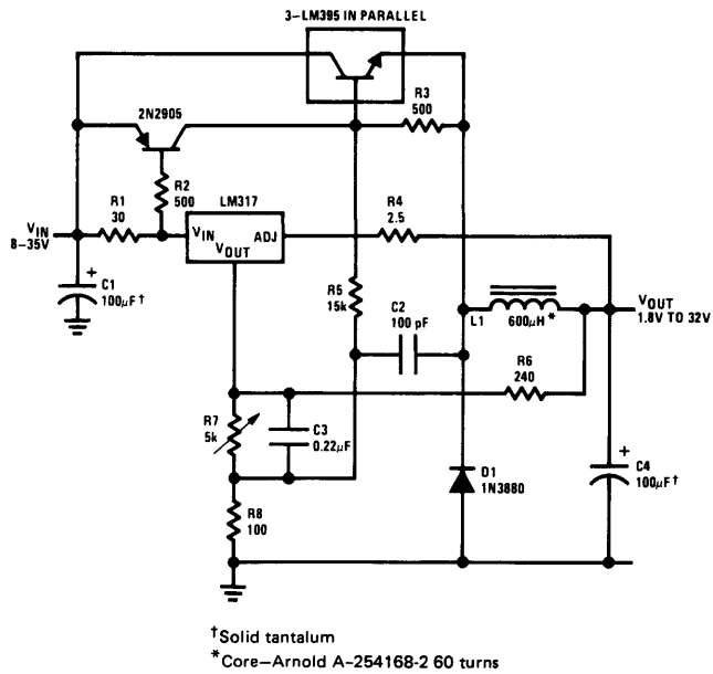
FIGURE 10. 4A Switching Regulator with Overload Protection
