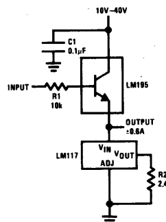
Power Follower
