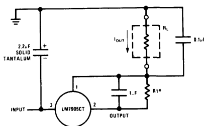
Current Source
