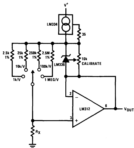
Linear Ohmmeter
