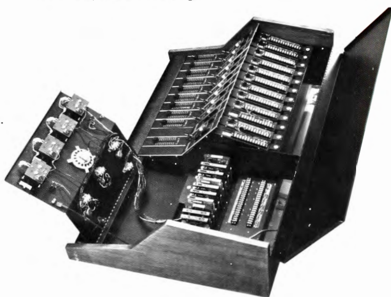
Model SL-4100 with top and right-hand front panels open. Input cabling readily terminated on input module top barrier strips. Output barrier strips at lower right. System plug-in electronic modules and secondary front panel controls and switches readily accessible. Installation eliminates all exposed cabling.
