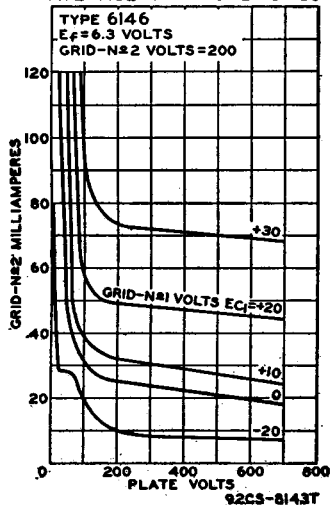
AVERAGE CHARACTERISTICS
