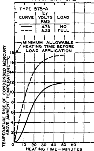
RATE OF RISE OF CONDENSED - MERCURY TEMPERATURE
