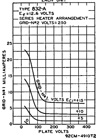
AVERAGE CHARACTERISTICS EACH UNIT
