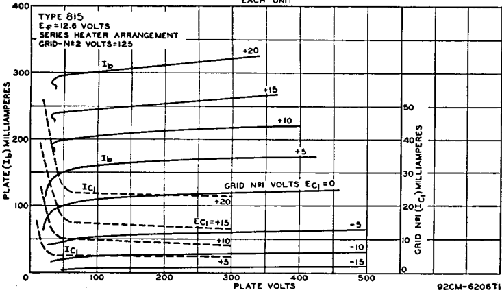
AVERAGE CHARACTERISTICS EACH UNIT
