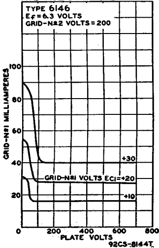
AVERAGE CHARACTERISTICS
