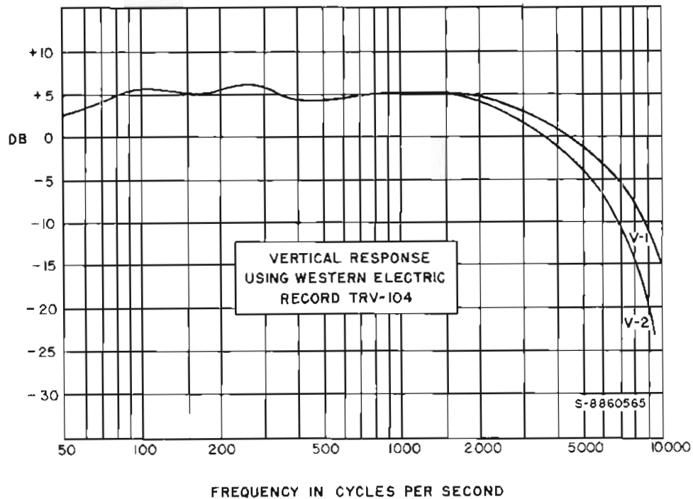
Figure 8—Overall frequency response for vertical switch positions using test record.
