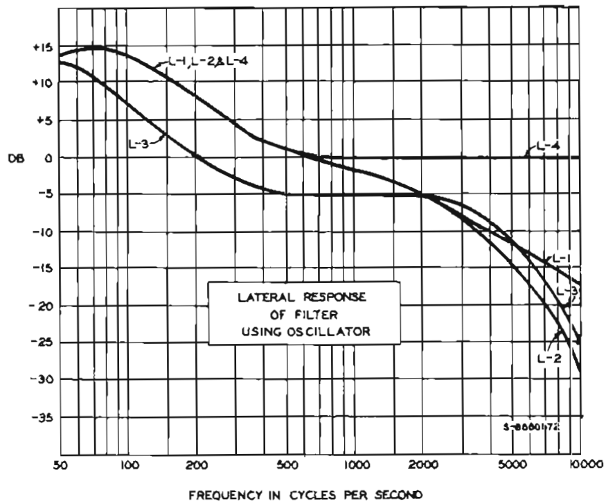
Figure 9—Frequency response of filter for lateral switch positions using oscillator.
