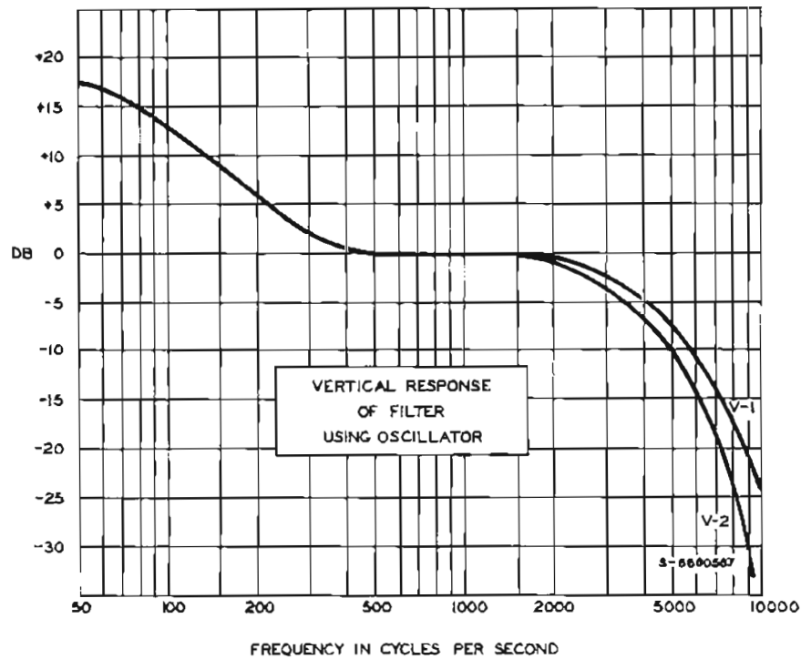
Figure 10—Frequency response of filter for vertical switch positions using oscillator.
