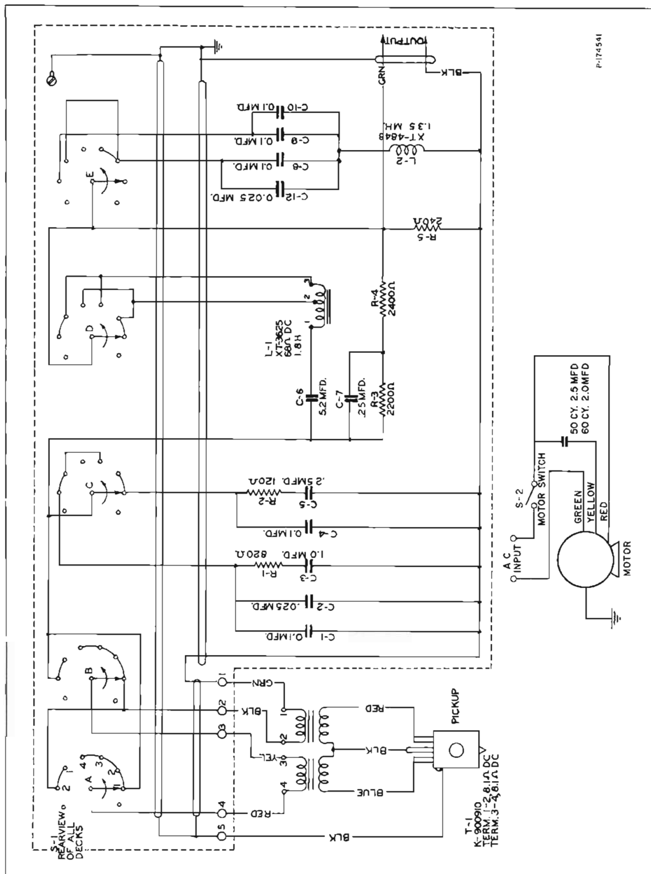
Figure 5—Schematic diagram.
